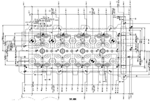
Component Drawing (Cover contact face)
