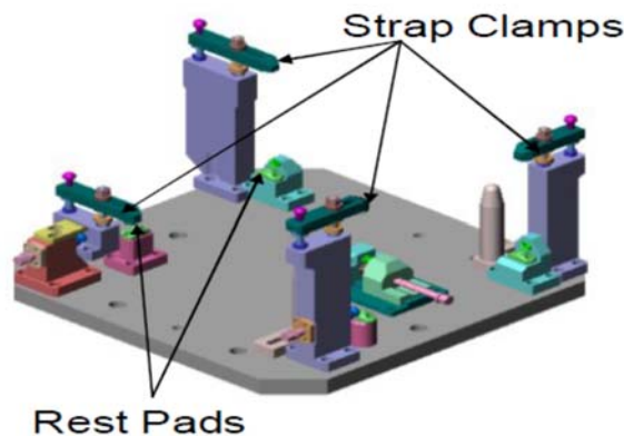
Fig 1.1: Mechanical Fixture
