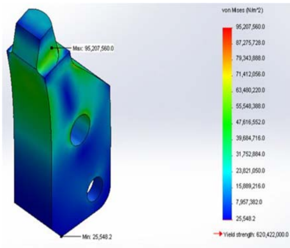
Fig. Static stress plot for link 2
