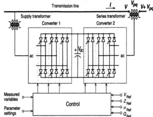
Fig 2. UPFC Control Structure
