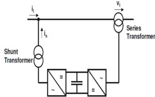
Fig 1. Principle Configuration of UPFC
